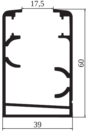
9133 - 1,108 kg/m
