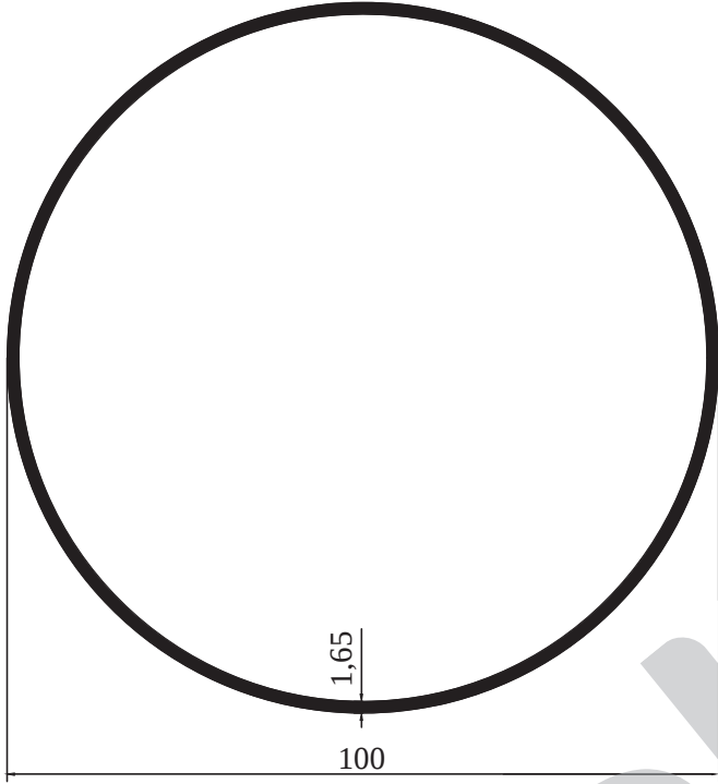
M 9525 - 1,381 kg/m
