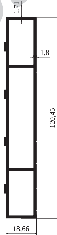
M 2323 - 1,126 kg/m
