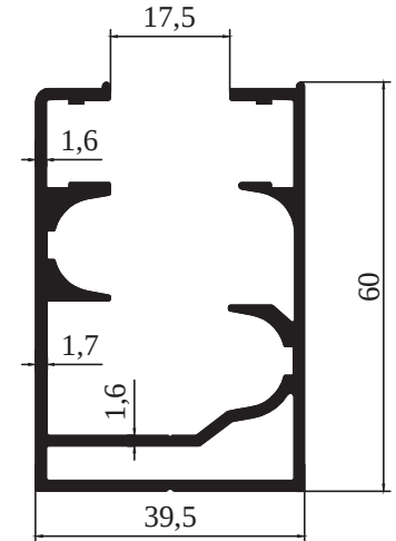
8193 - 1,198 kg/m
