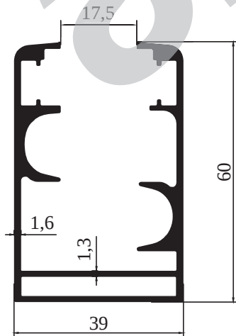
M 2106 - 1,218 kg/m
