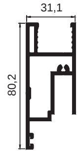
M 2493 - 1.028 kg/m
