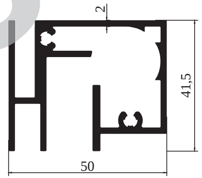
M 2475 - 1,420 kg/m
