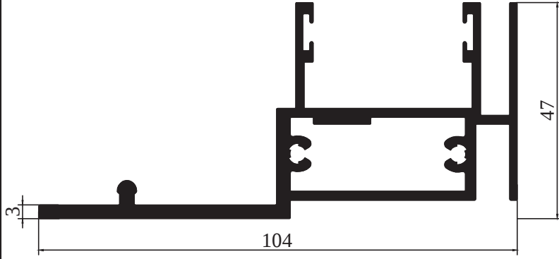
M 2476 - 1,873 kg/m
