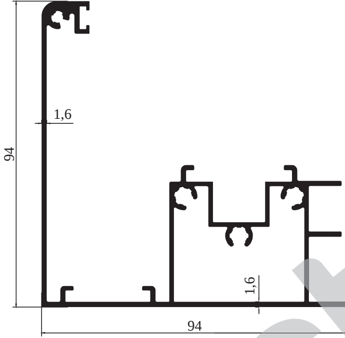
M 9510 - 1,891 kg/m
