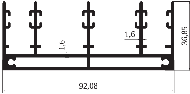
M 2301 - 1,184 kg/m
